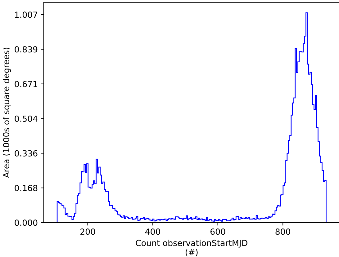
ddf_loaded_fl1_v3.4_10yrs : Count observationStartMJD
