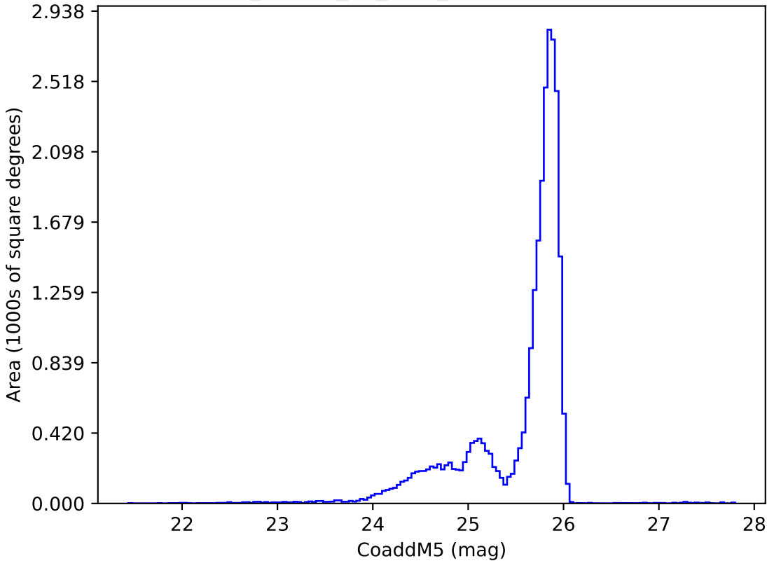
ddf_loaded_fl1_v3.4_10yrs z: CoaddM5
