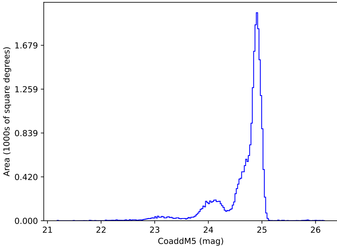
ddf_loaded_fl1_v3.4_10yrs y: CoaddM5
