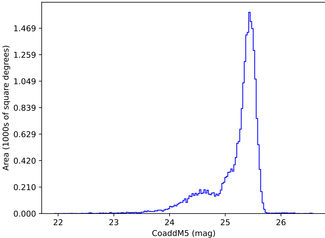
ddf_loaded_fl1_v3.4_10yrs u: CoaddM5
