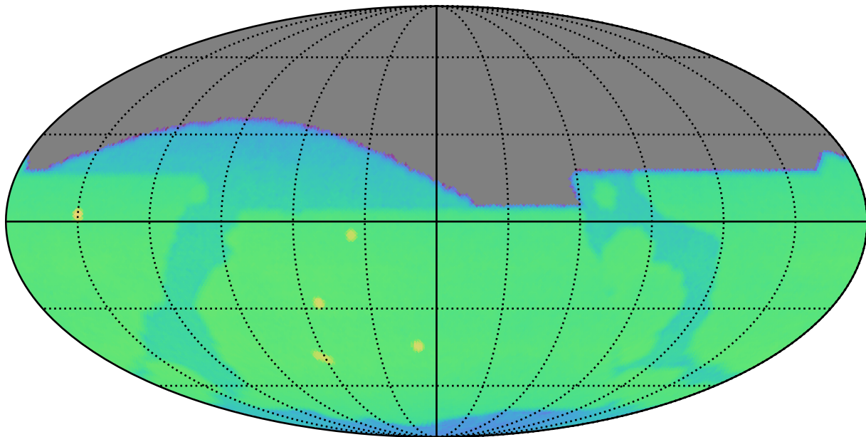
ddf_loaded_fl1_v3.4_10yrs r: CoaddM5
