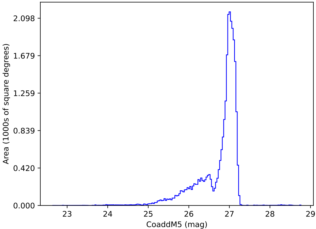
ddf_loaded_fl1_v3.4_10yrs r: CoaddM5
