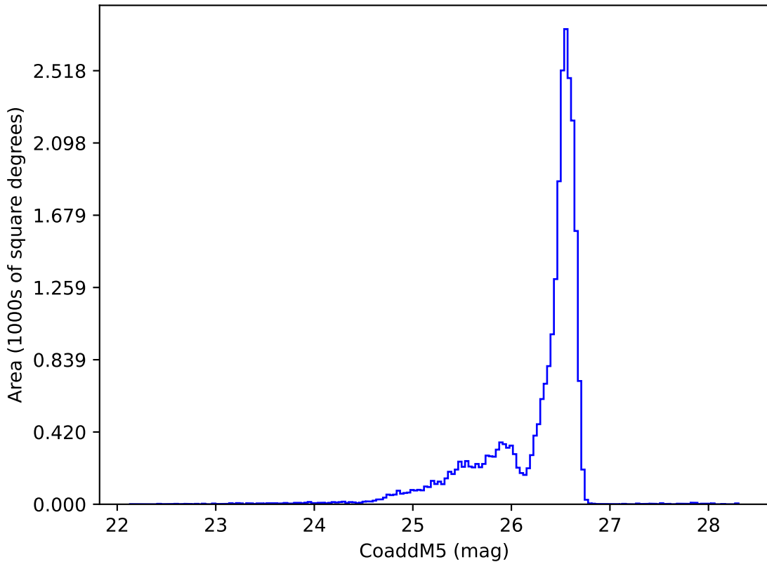
ddf_loaded_fl1_v3.4_10yrs i: CoaddM5
