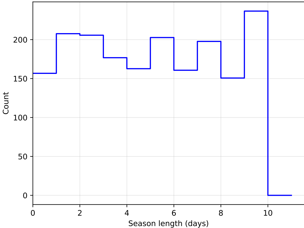
ddf_loaded_fl1_v3.4_10yrs DD:WFD all bands: SeasonLength
