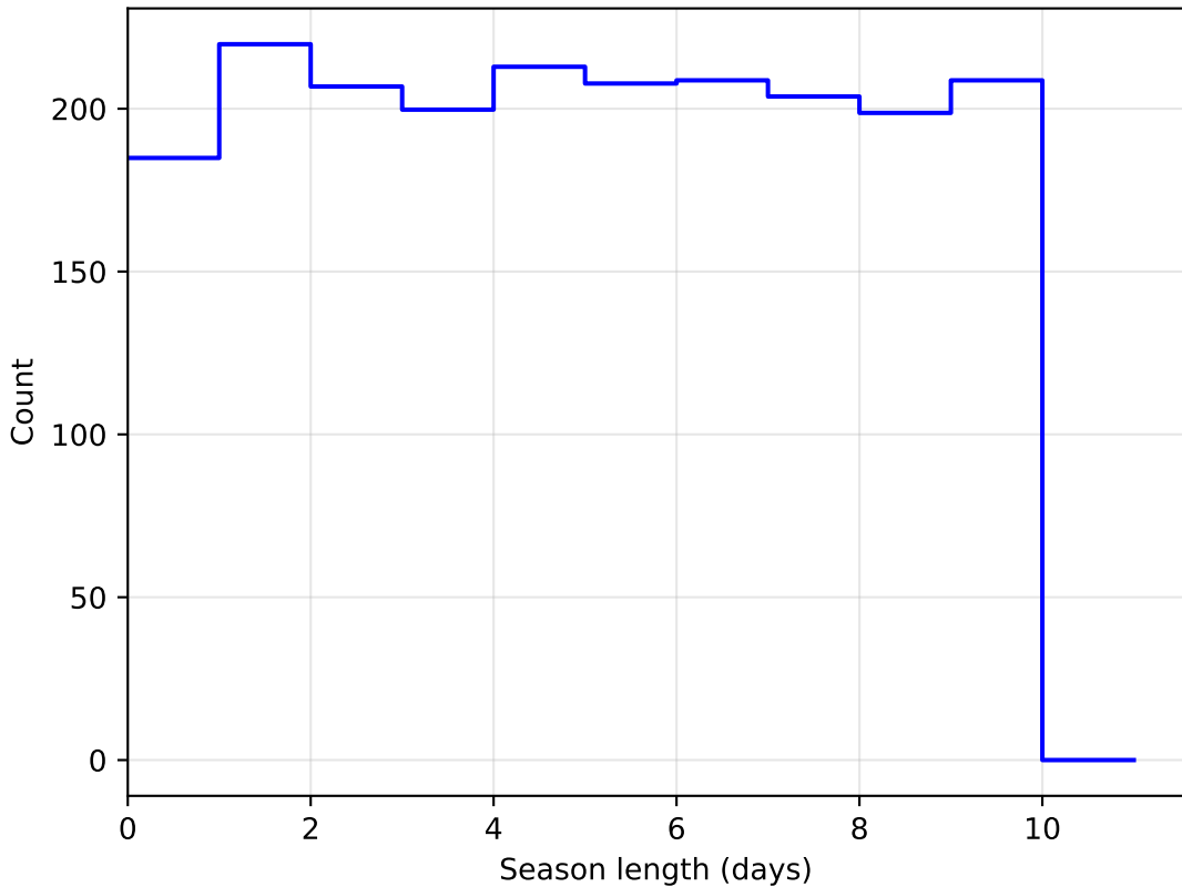
ddf_loaded_fl1_v3.4_10yrs DD:ELAISS1 all bands: SeasonLength
