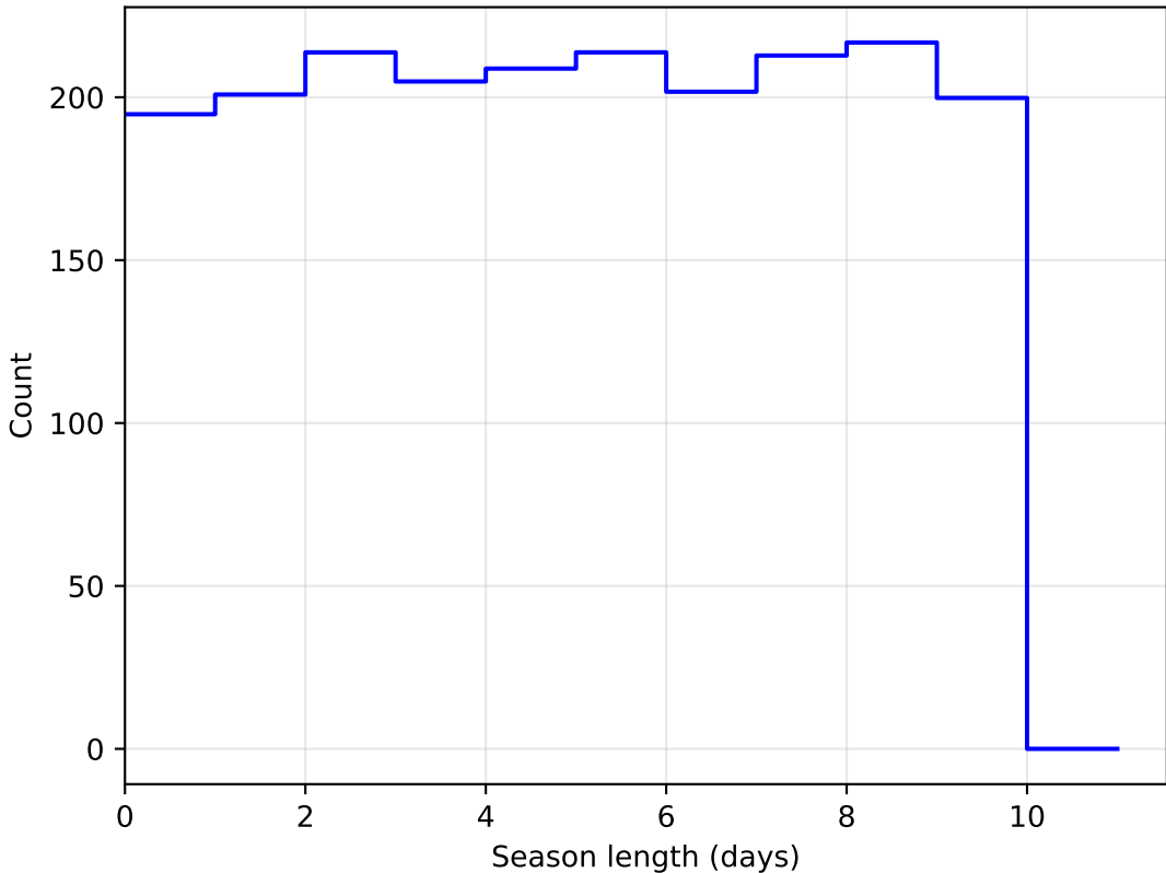
ddf_loaded_fl1_v3.4_10yrs DD:ECDFS all bands: SeasonLength
