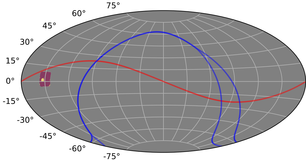
0.0 0.1 0.2 0.3 0.4 0.5 0.6 0.7 0.8 0.9 1.0 KNePopMetric_DD:COSMOS_ztfrest_simple_red (Detected, 0 or 1)
