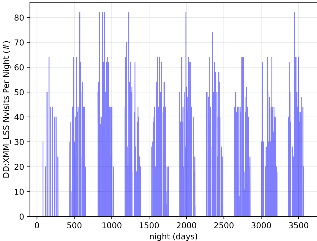
ddf_loaded_fl1_v3.4_10yrs all bands: DD:XMM_LSS Nvisits Per Night
