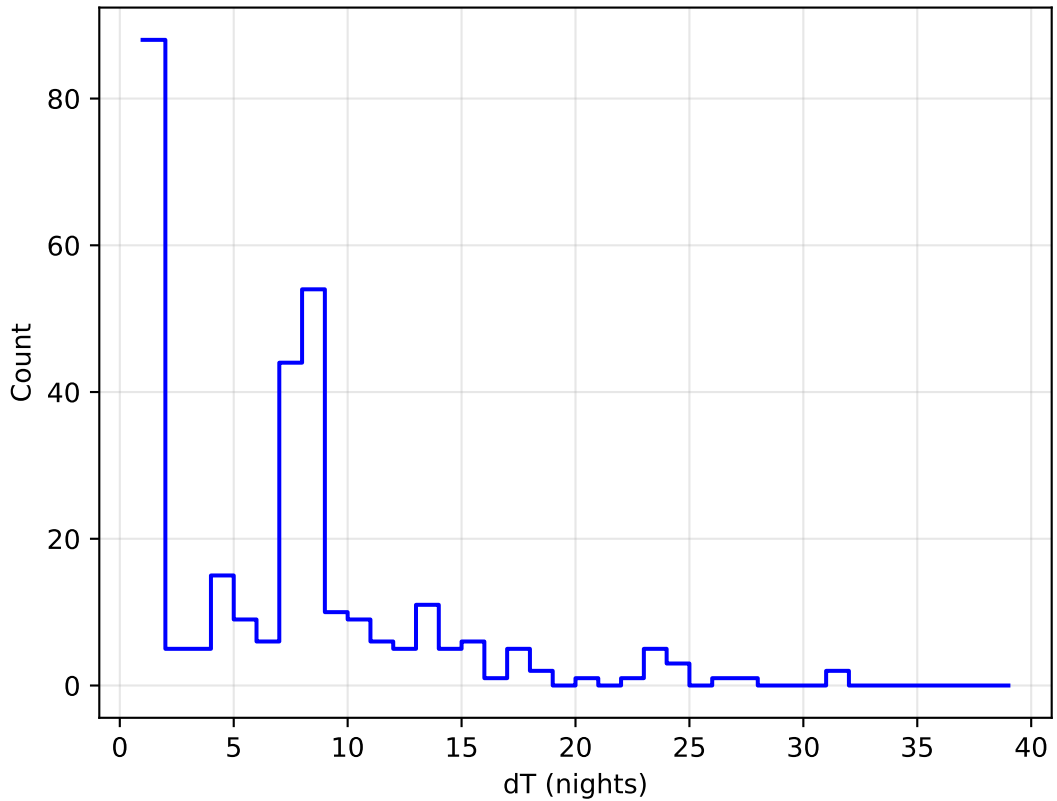
ddf_loaded_fl1_v3.4_10yrs all bands: DD:XMM_LSS Delta Nights Histogram
