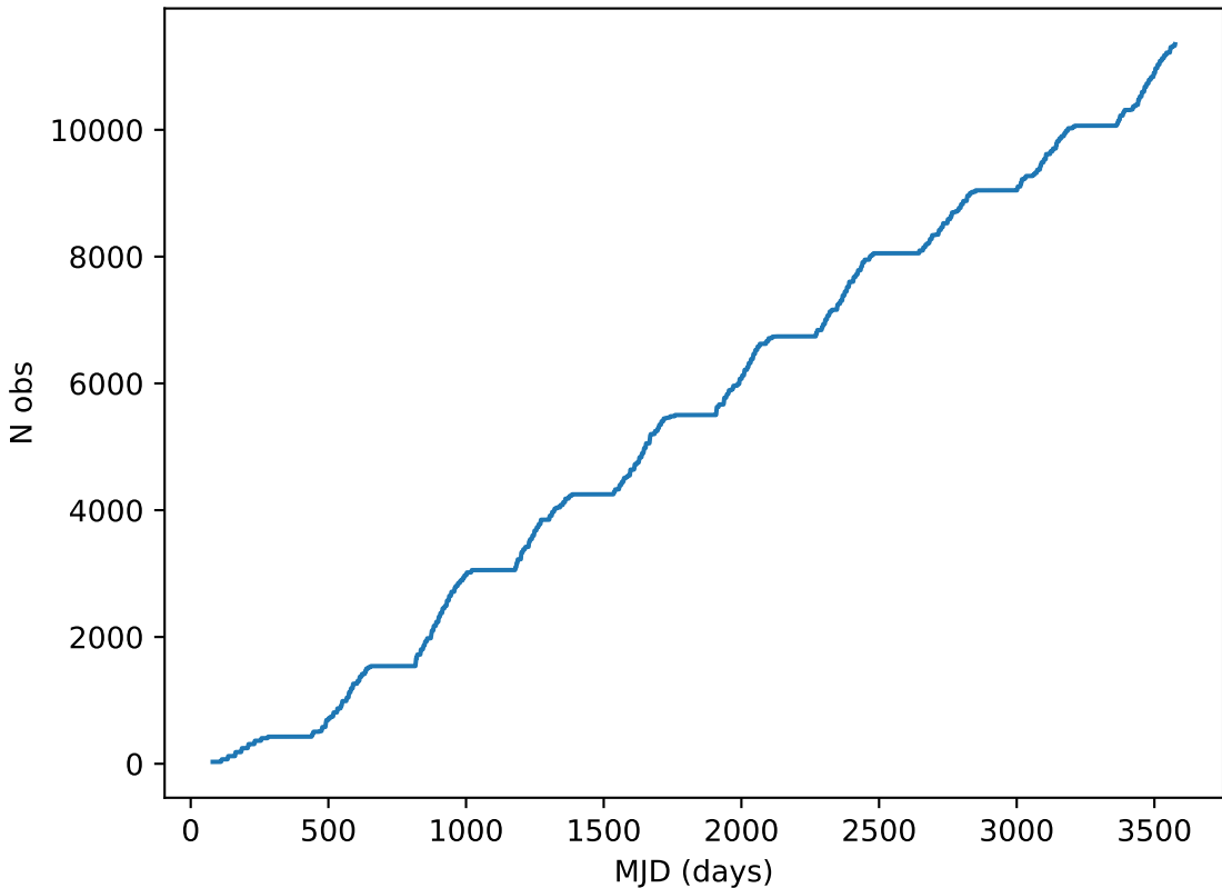
ddf_loaded_fl1_v3.4_10yrs all bands: DD:XMM_LSS Cumulative NVisits
