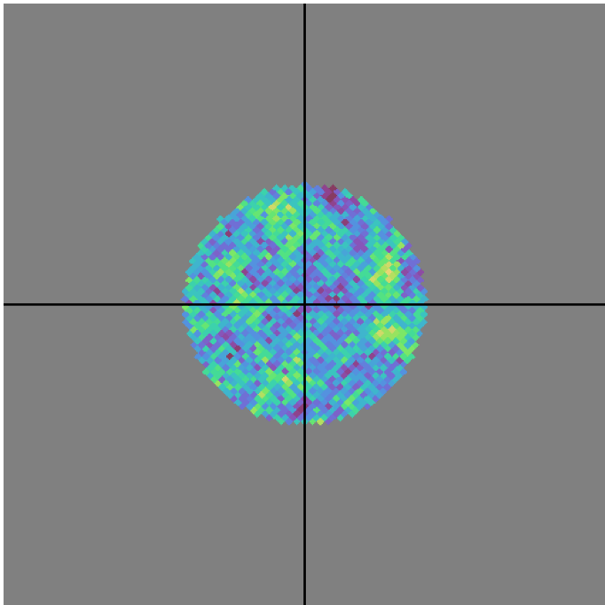
ddf_loaded_fl1_v3.4_10yrs u band: DD:WFD NVisits
