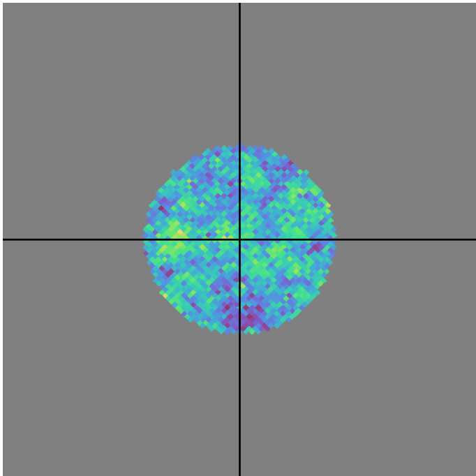
ddf_loaded_fl1_v3.4_10yrs g band: DD:WFD NVisits
