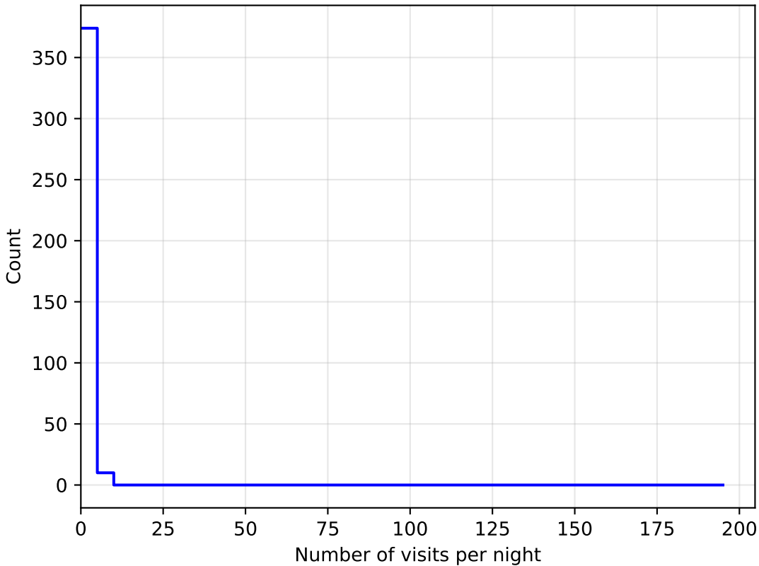
ddf_loaded_fl1_v3.4_10yrs all bands: DD:WFD NVisitsPerNight
