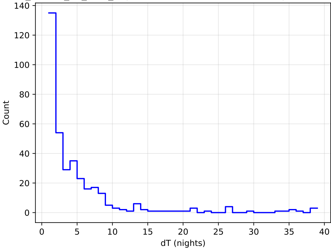
ddf_loaded_fl1_v3.4_10yrs all bands: DD:WFD Delta Nights Histogram
