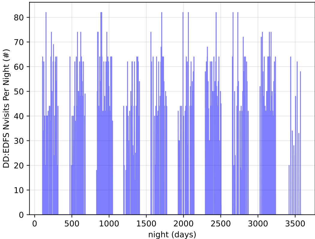
ddf_loaded_fl1_v3.4_10yrs all bands: DD:EDFS Nvisits Per Night
