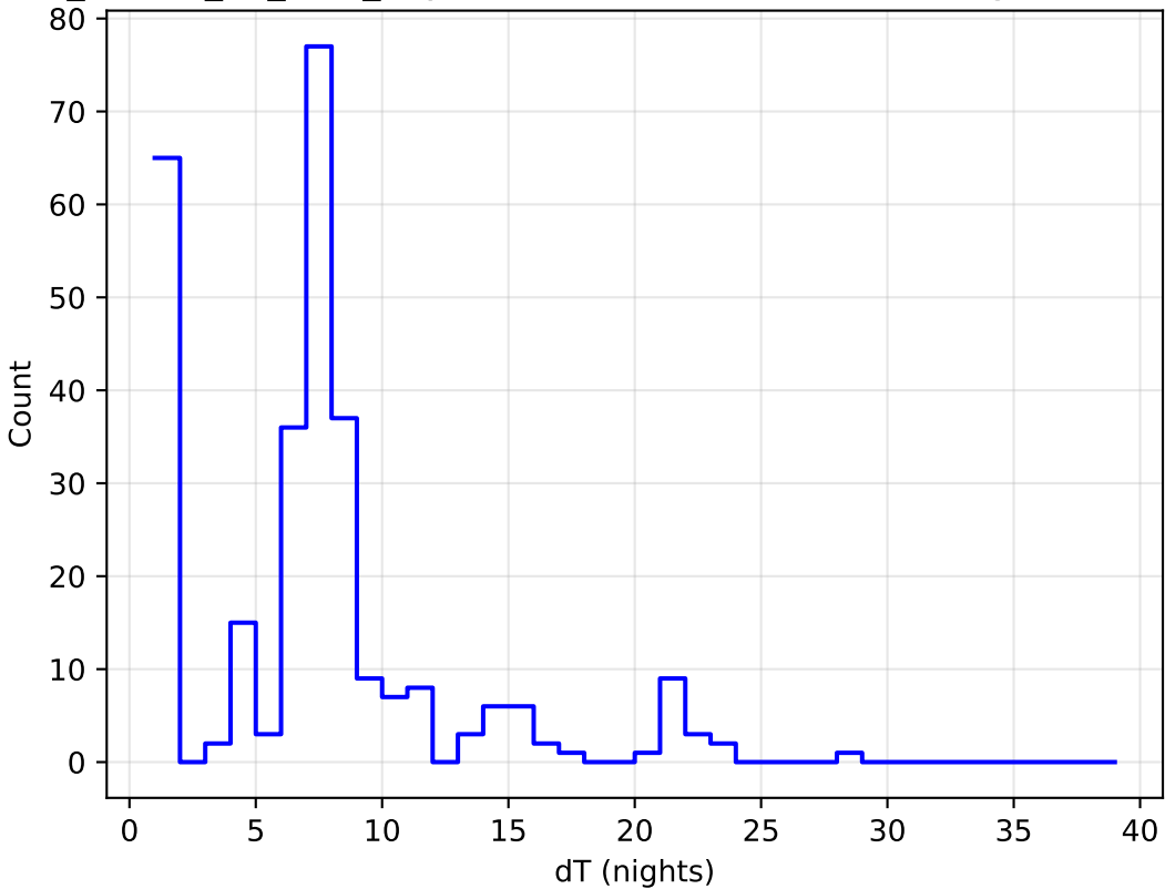
ddf_loaded_fl1_v3.4_10yrs all bands: DD:EDFS Delta Nights Histogram
