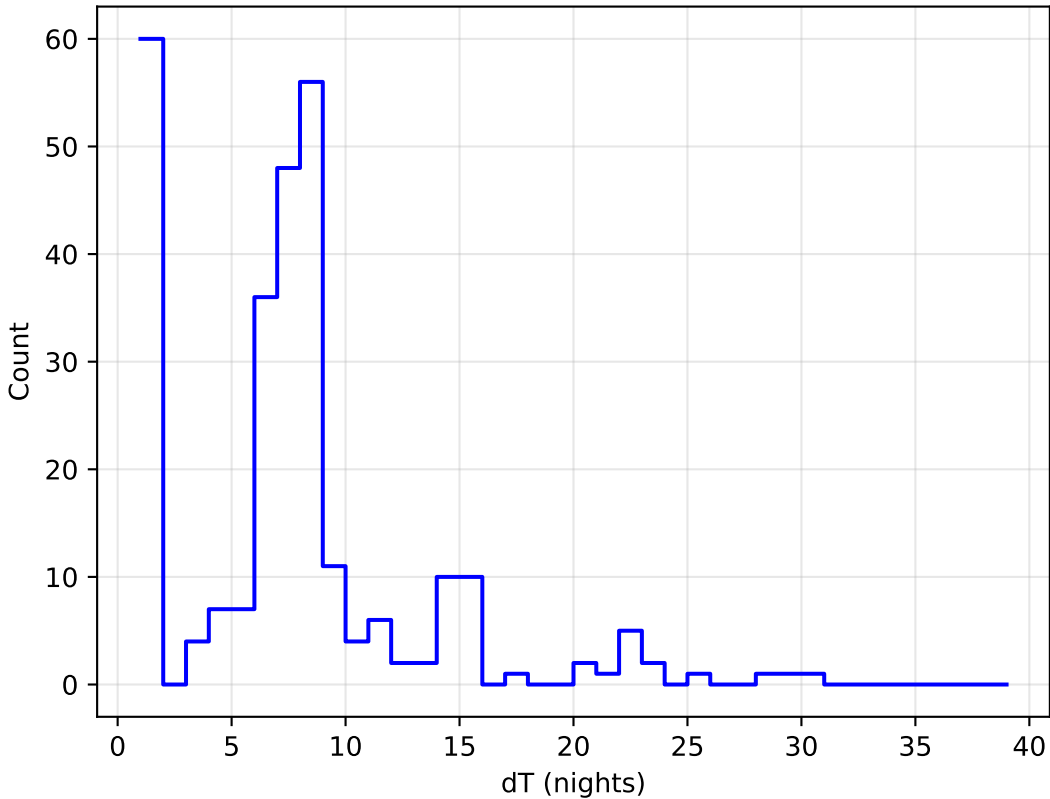
ddf_loaded_fl1_v3.4_10yrs all bands: DD:ECDFS Delta Nights Histogram
