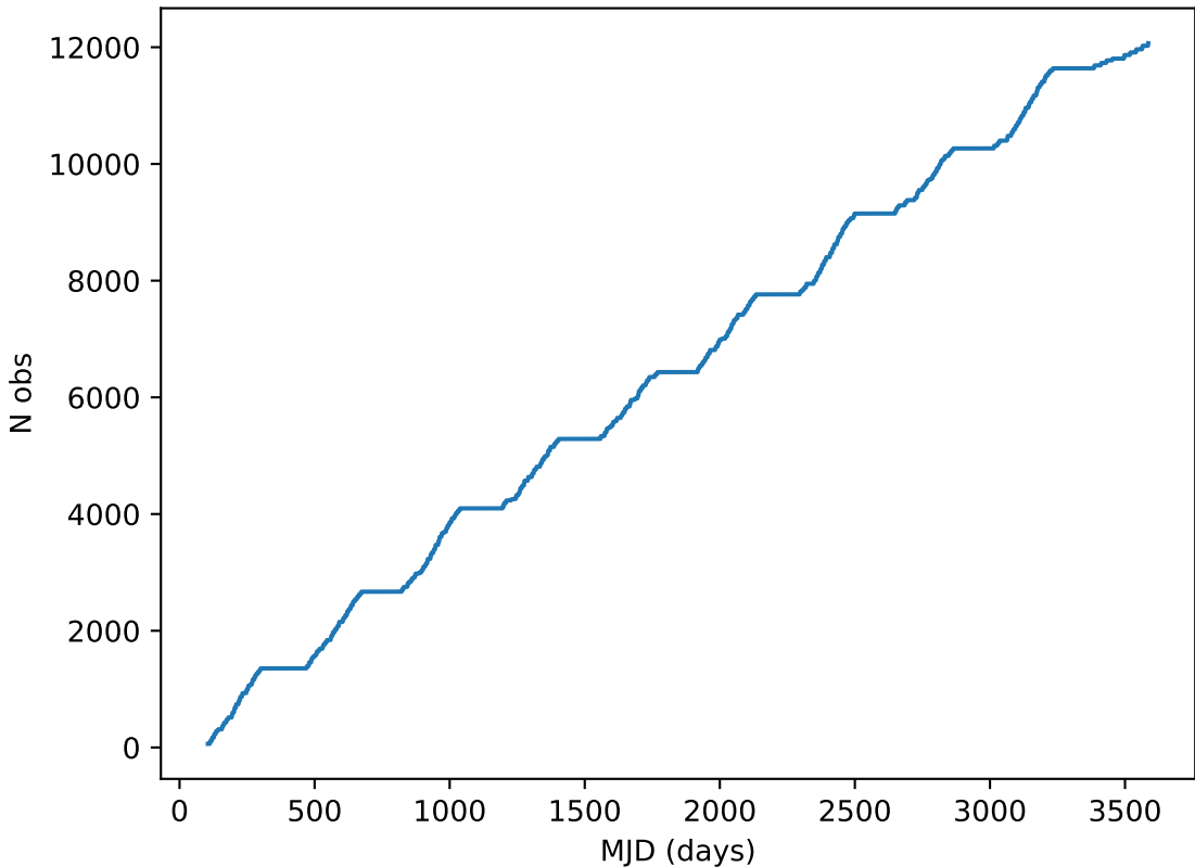
ddf_loaded_fl1_v3.4_10yrs all bands: DD:ECDFS Cumulative NVisits
