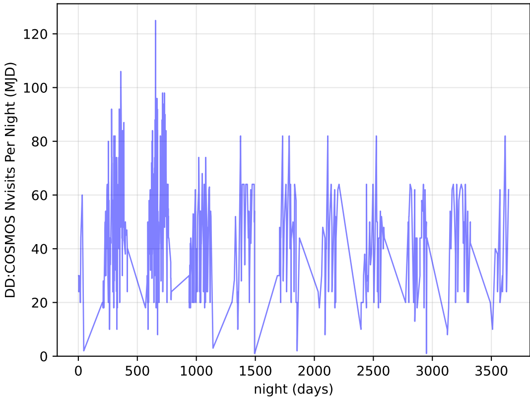
ddf_loaded_fl1_v3.4_10yrs all bands: DD: COSMOS Nvisits Per Night
