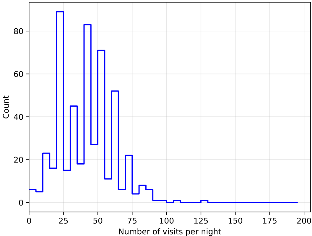
ddf_loaded_fl1_v3.4_10yrs all bands: DD:COSMOS NVisitsPerNight
