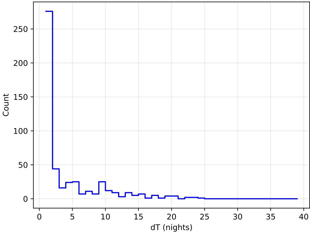
ddf_loaded_fl1_v3.4_10yrs all bands: DD: COSMOS Delta Nights Histogram
