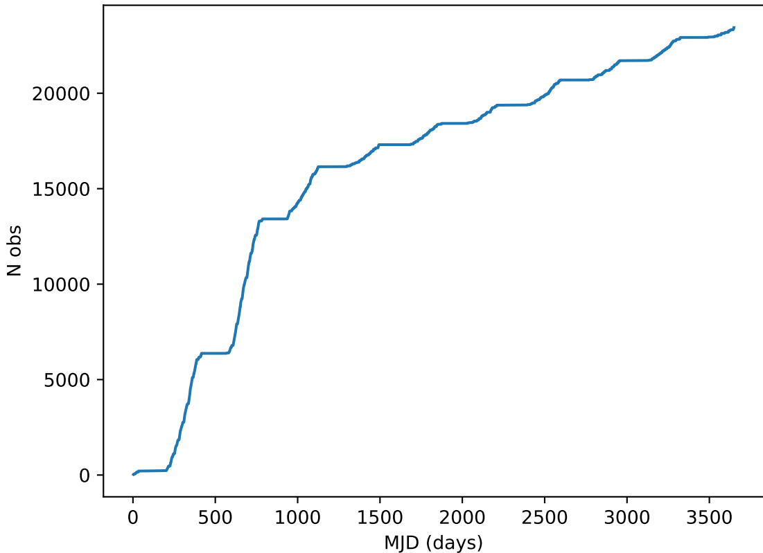
ddf_loaded_fl1_v3.4_10yrs all bands: DD:COSMOS Cumulative NVisits
