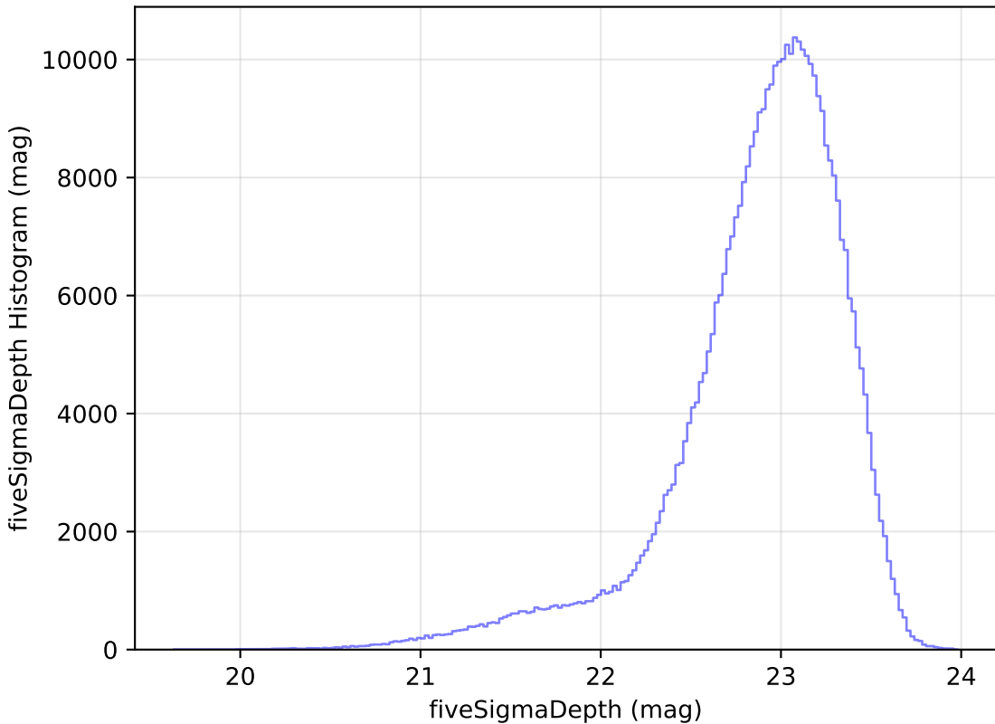
ddf_loaded_fl1_v3.3_10yrs z: fiveSigmaDepth Histogram
