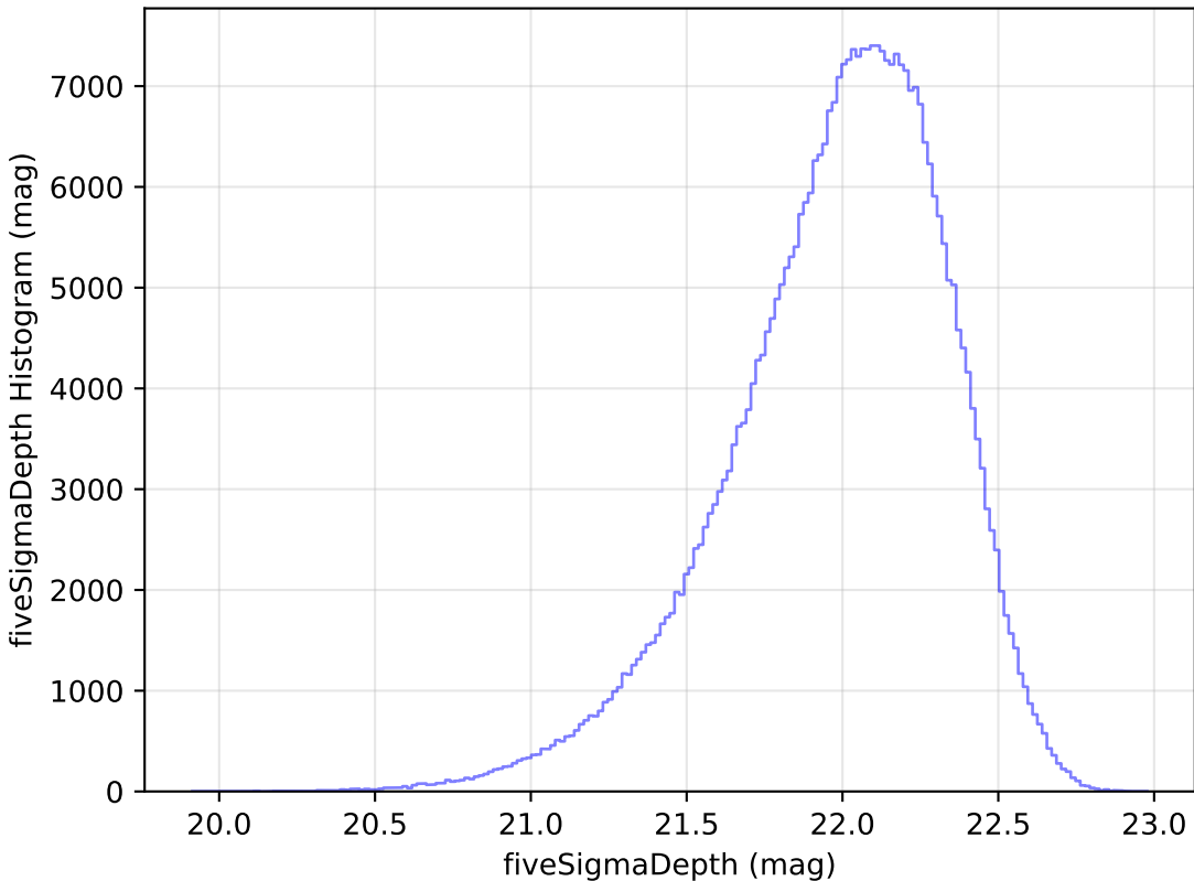
ddf_loaded_fl1_v3.3_10yrs y: fiveSigmaDepth Histogram
