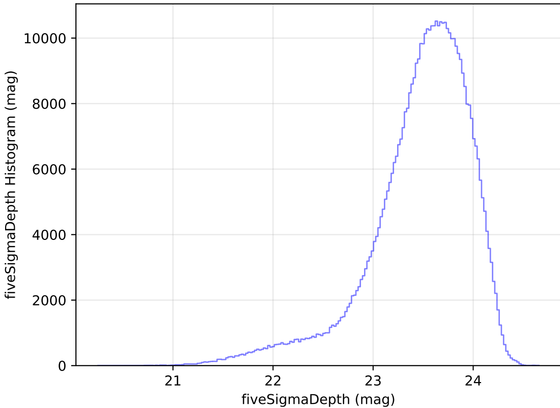
ddf_loaded_fl1_v3.3_10yrs i: fiveSigmaDepth Histogram
