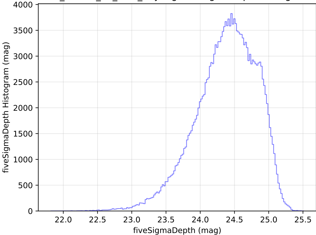
ddf_loaded_fl1_v3.3_10yrs g: fiveSigmaDepth Histogram
