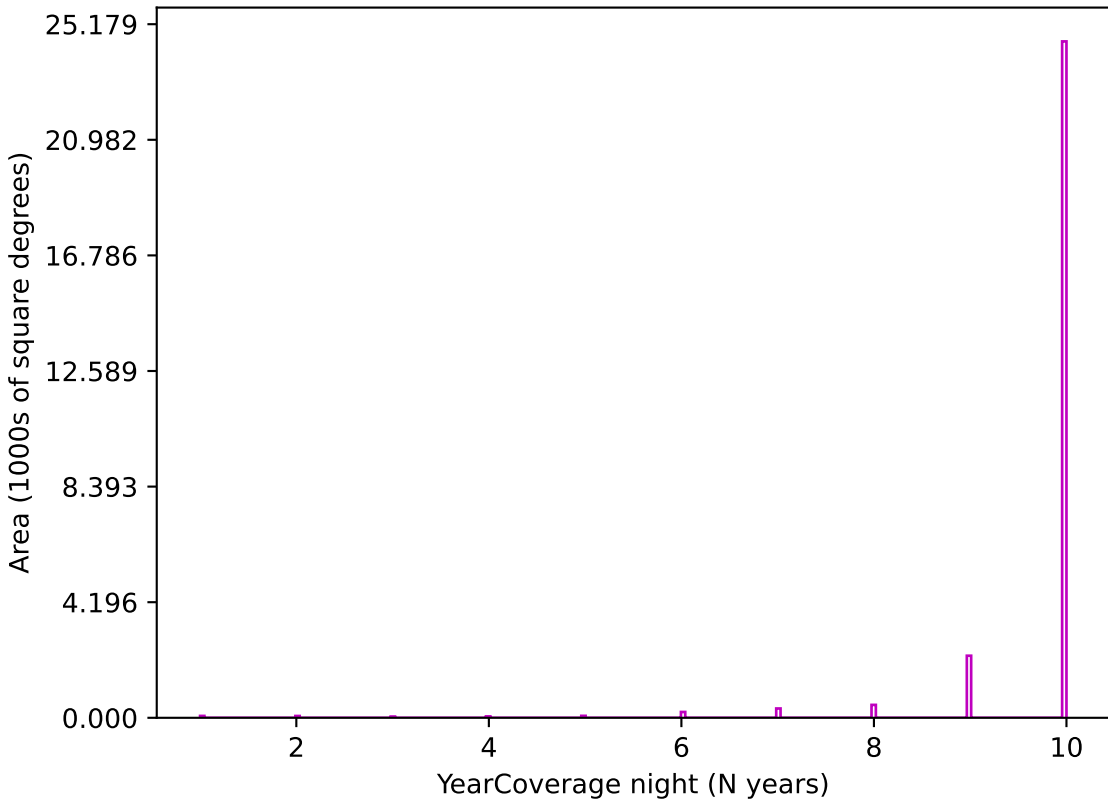
ddf_loaded_fl1_v3.3_10yrs z band: YearCoverage night
