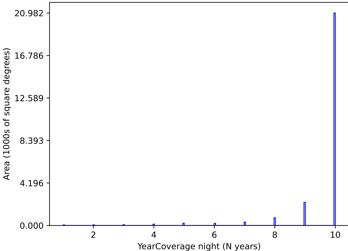
ddf_loaded_fl1_v3.3_10yrs y band: YearCoverage night
