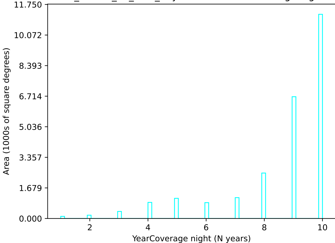
ddf_loaded_fl1_v3.3_10yrs u band: YearCoverage night
