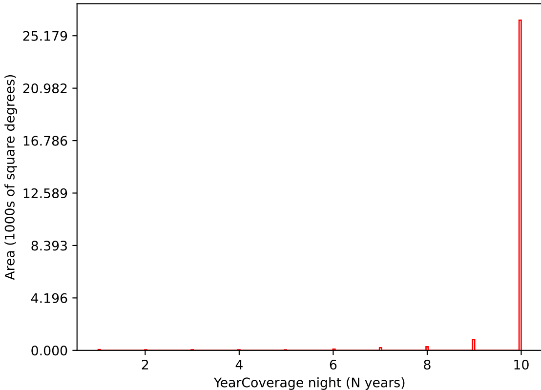
ddf_loaded_fl1_v3.3_10yrs i band: YearCoverage night
