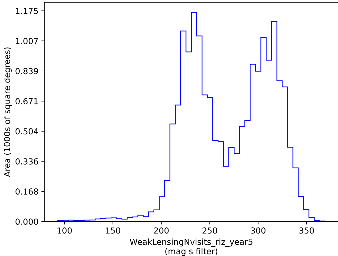
ddf_loaded_fl1_v3.3_10yrs gri band non-DD: WeakLensingNvisits_riz_year5
