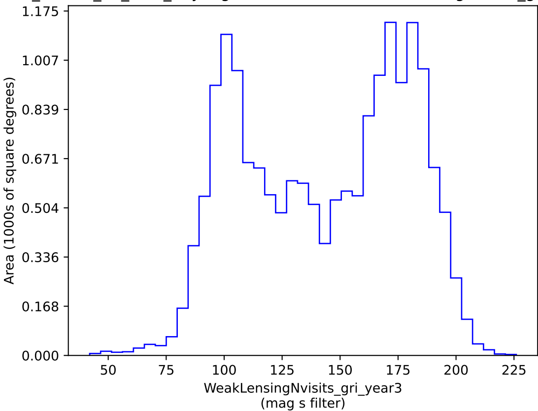
ddf_loaded_fl1_v3.3_10yrs gri band non-DD: WeakLensingNvisits_gri_year3
