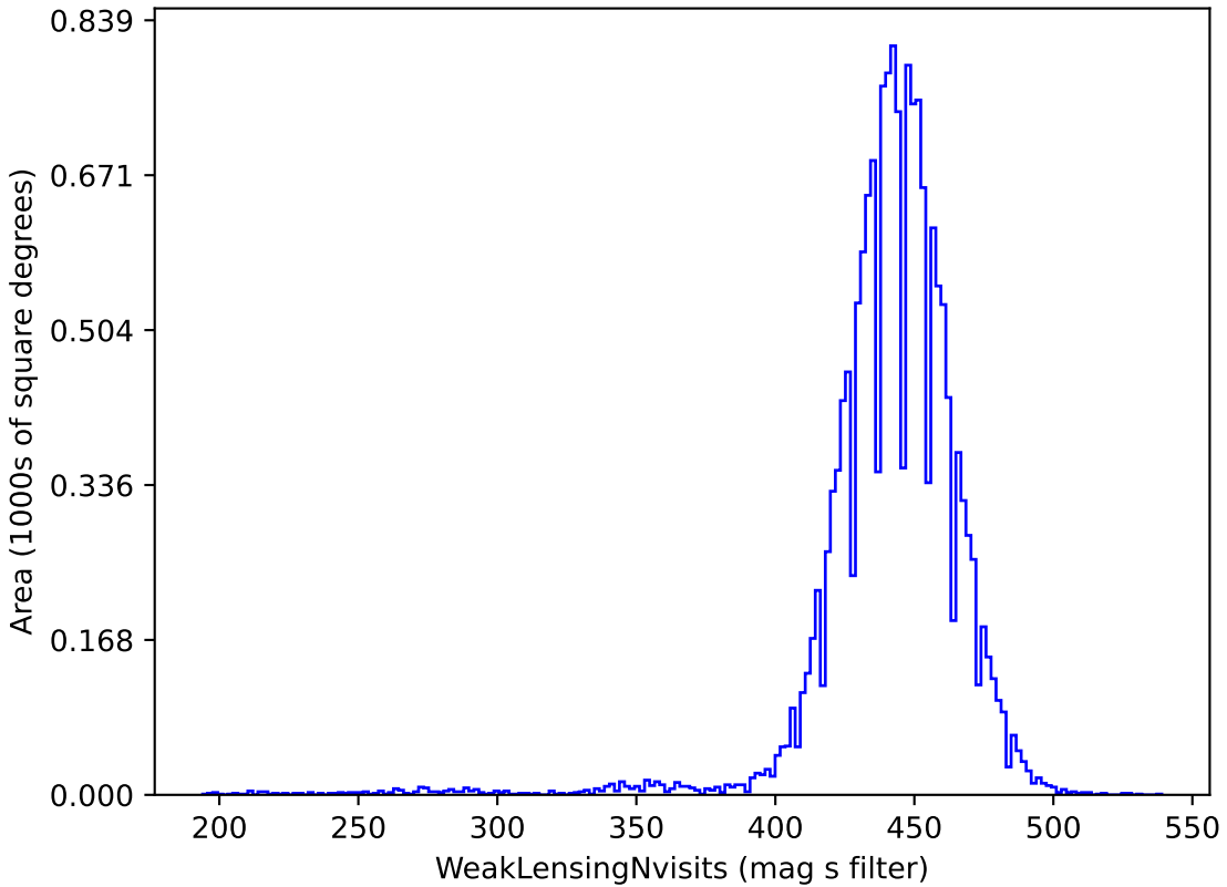
ddf_loaded_fl1_v3.3_10yrs gri band non-DD: WeakLensingNvisits
