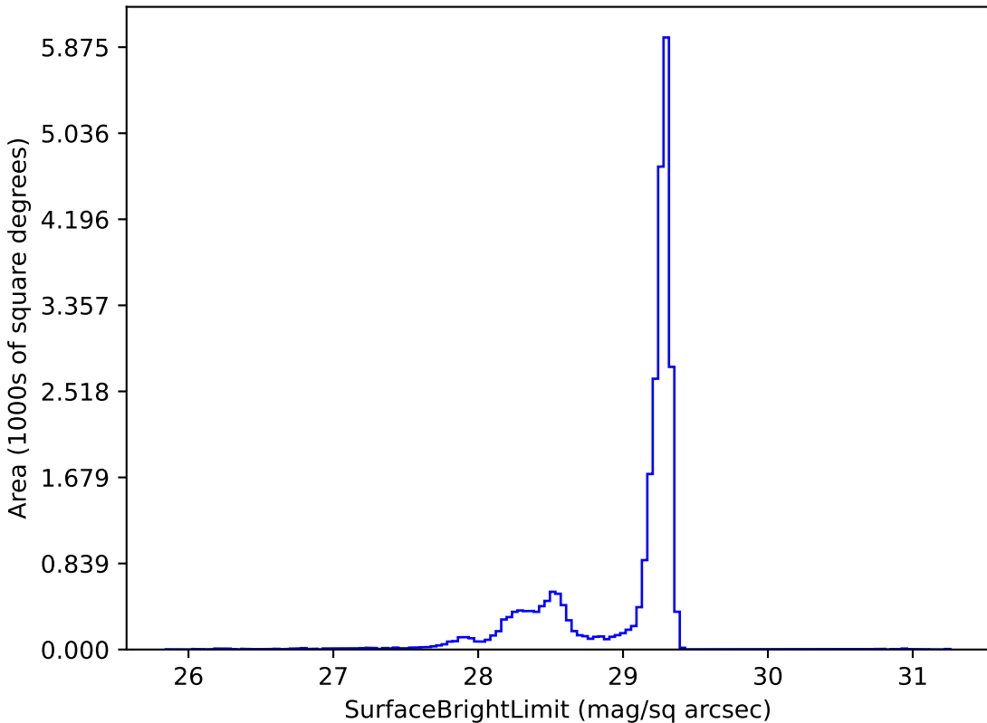
ddf_loaded_fl1_v3.3_10yrs z: SurfaceBrightLimit
