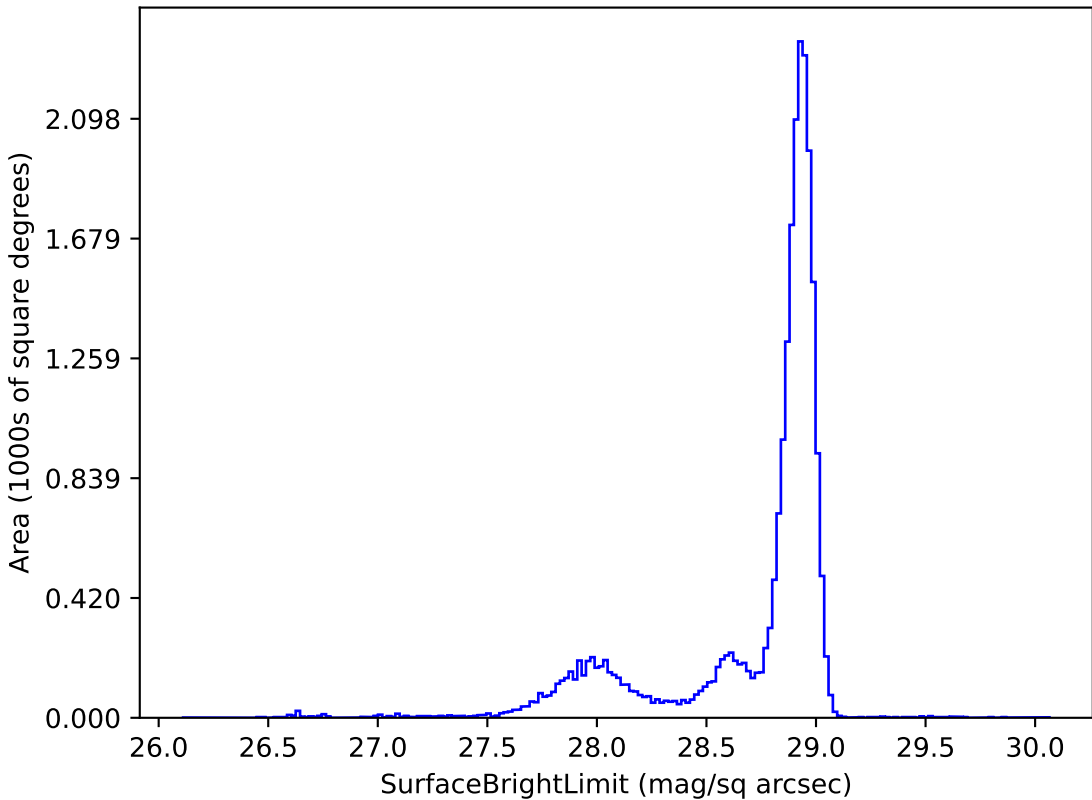
ddf_loaded_fl1_v3.3_10yrs u: SurfaceBrightLimit
