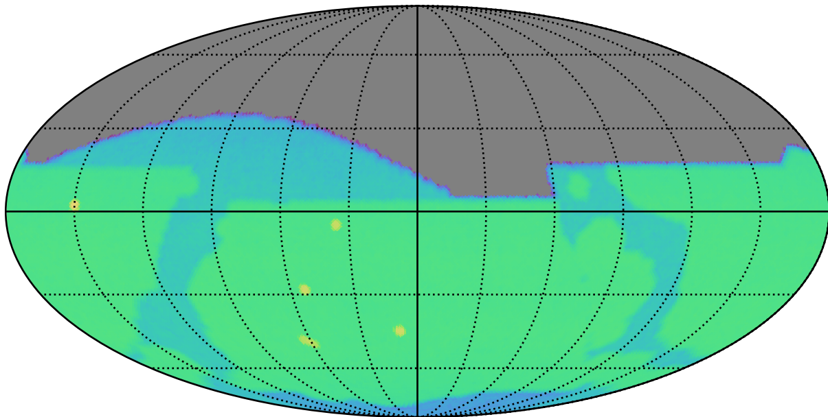
ddf_loaded_fl1_v3.3_10yrs i: SurfaceBrightLimit
