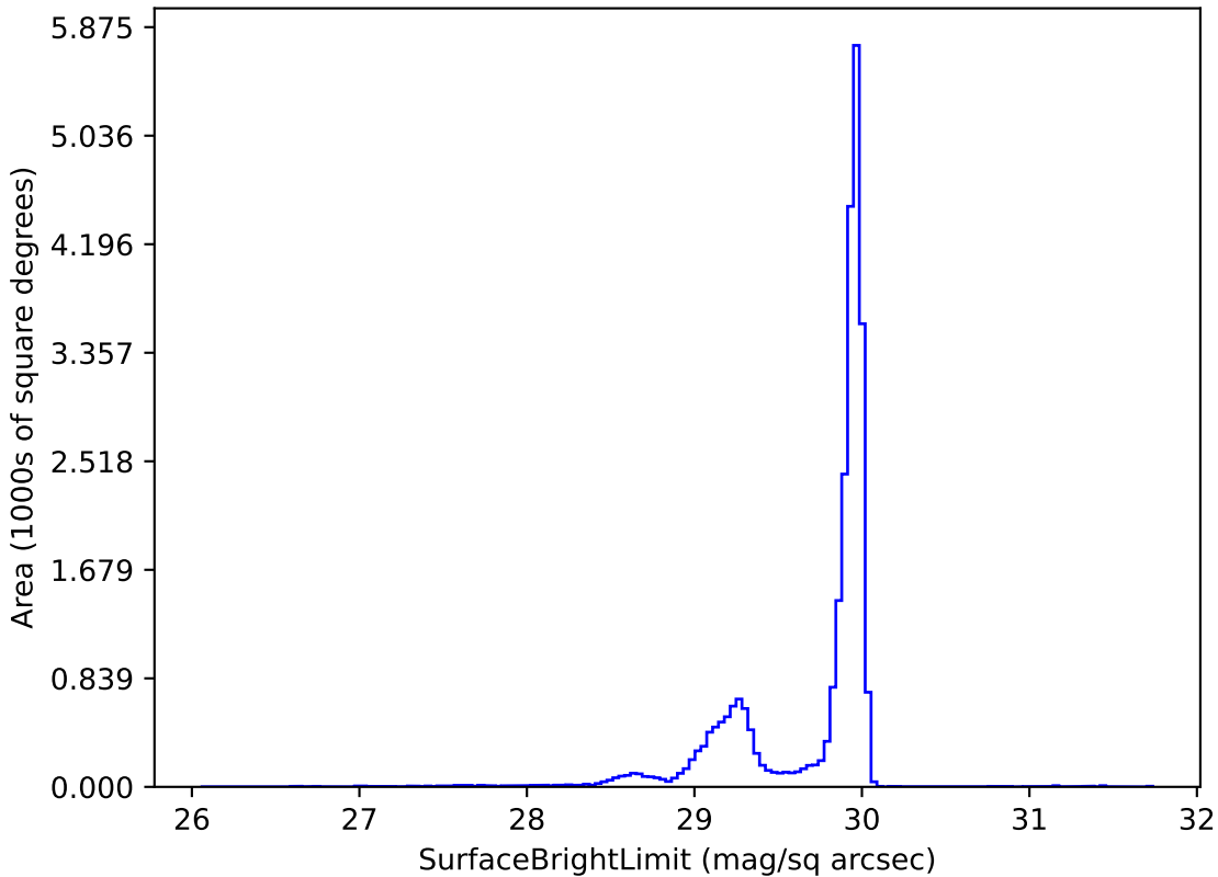
ddf_loaded_fl1_v3.3_10yrs i: SurfaceBrightLimit
