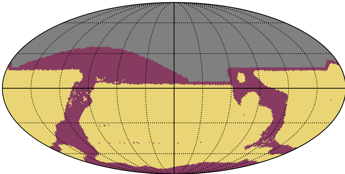
ddf_loaded_fl1_v3.3_10yrs : RapidRevisits
