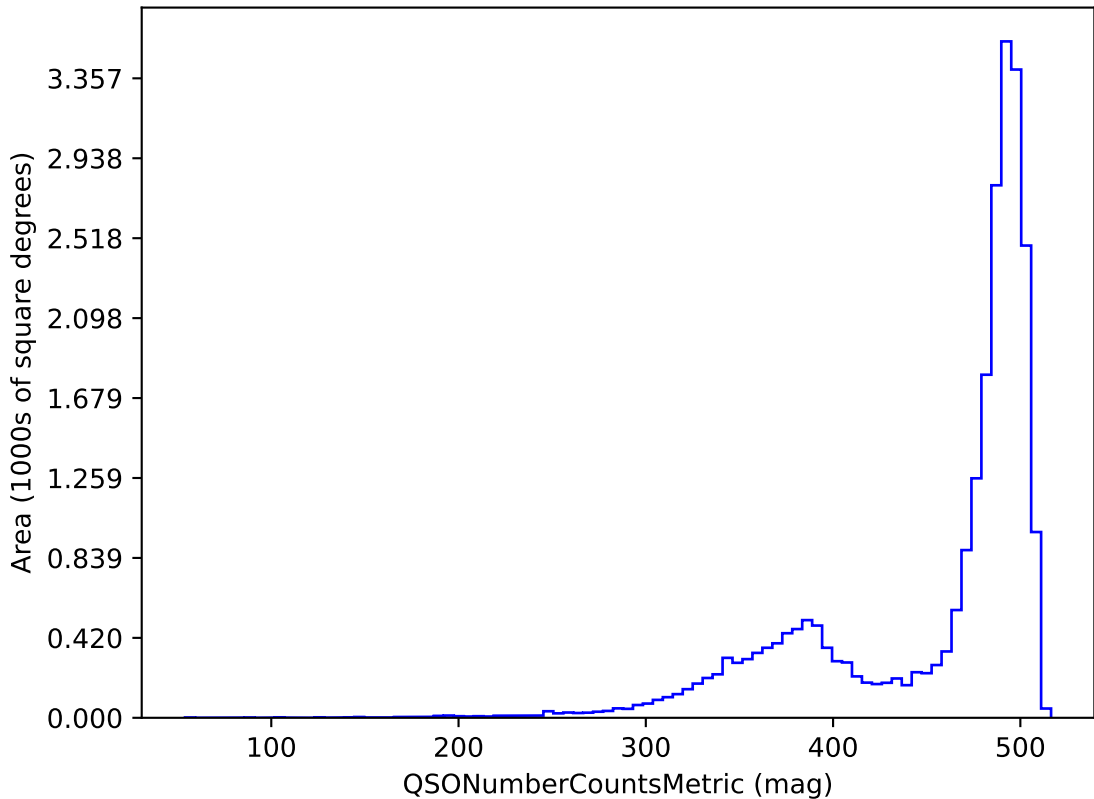
ddf_loaded_fl1_v3.3_10yrs z band and non-DD: QSONumberCountsMetric
