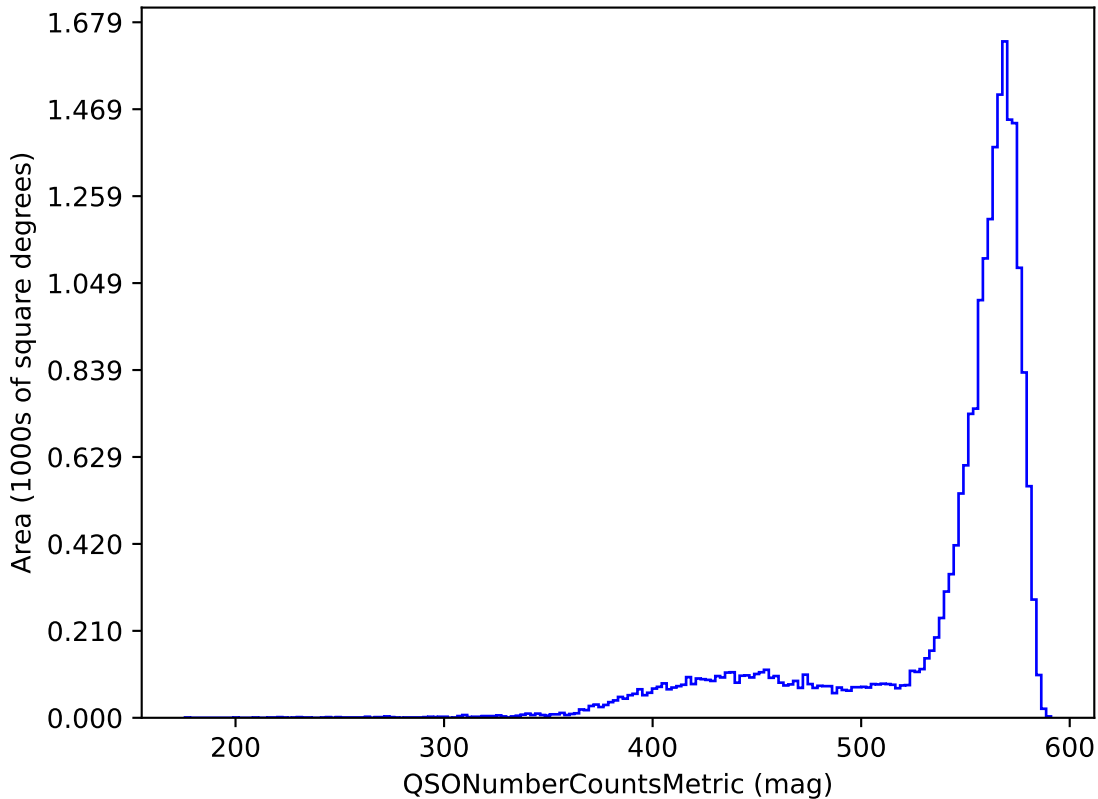
ddf_loaded_fl1_v3.3_10yrs y band and non-DD: QSONumberCountsMetric
