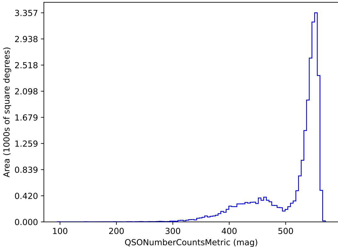
ddf_loaded_fl1_v3.3_10yrs i band and non-DD: QSONumberCountsMetric
