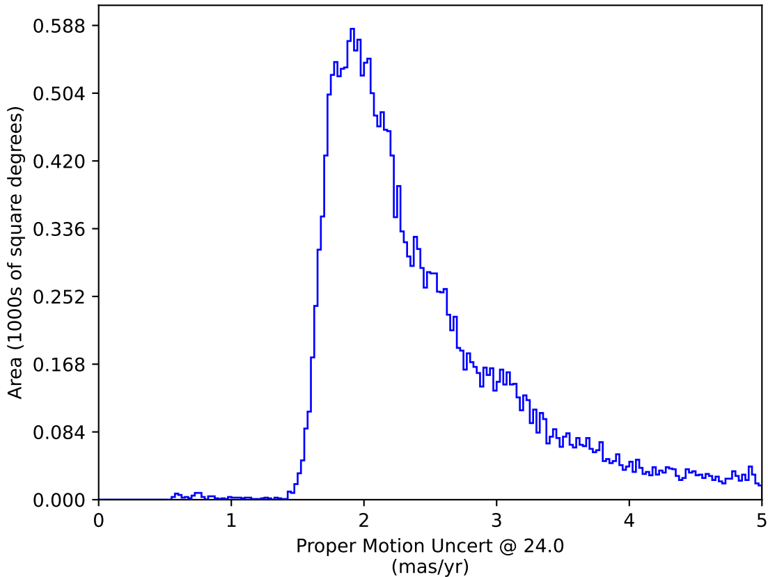
ddf_loaded_fl1_v3.3_10yrs : Proper Motion Uncert @ 24.0
