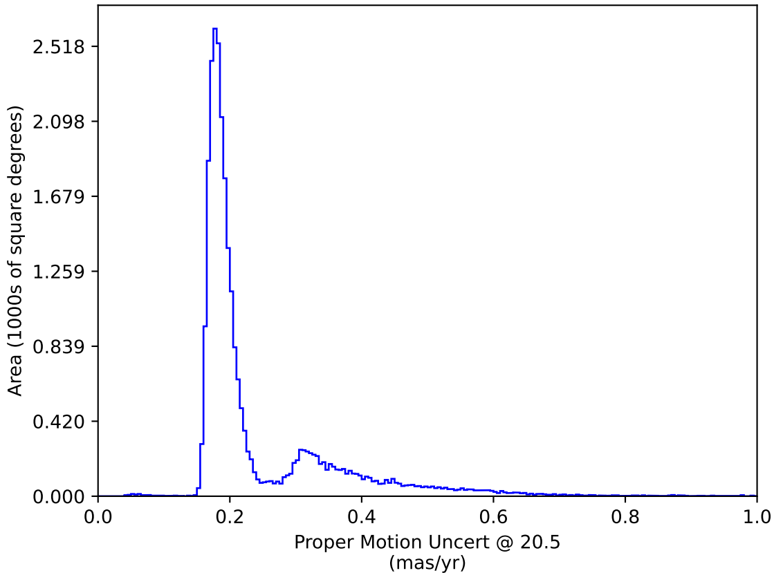
ddf_loaded_fl1_v3.3_10yrs : Proper Motion Uncert @ 20.5
