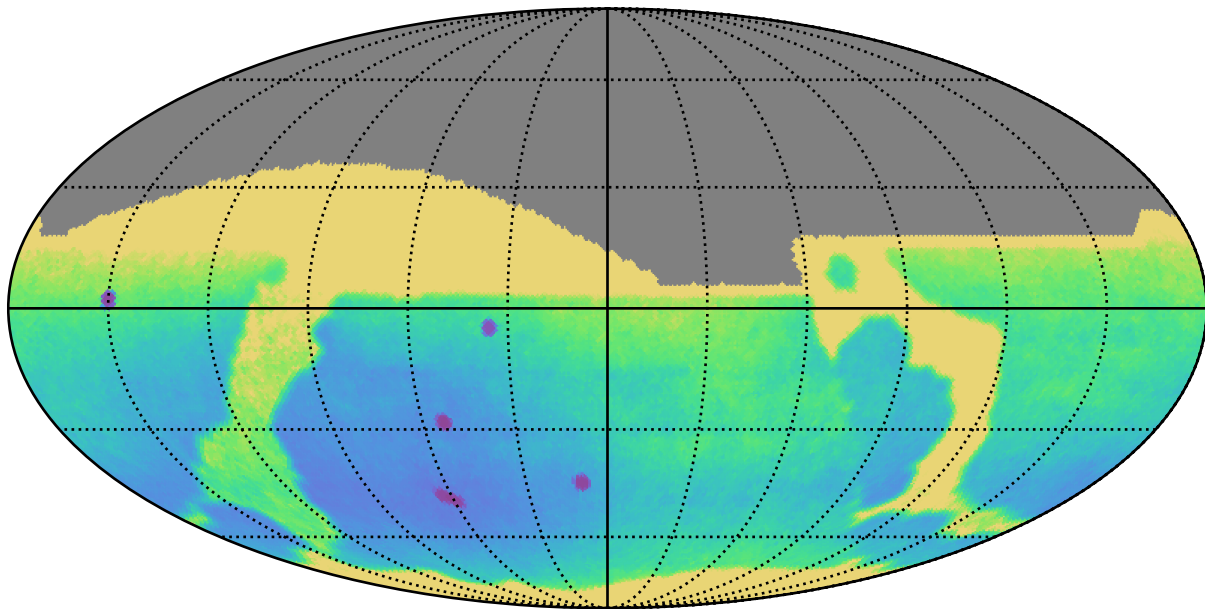
ddf_loaded_fl1_v3.3_10yrs : Parallax Uncert @ 24.0
