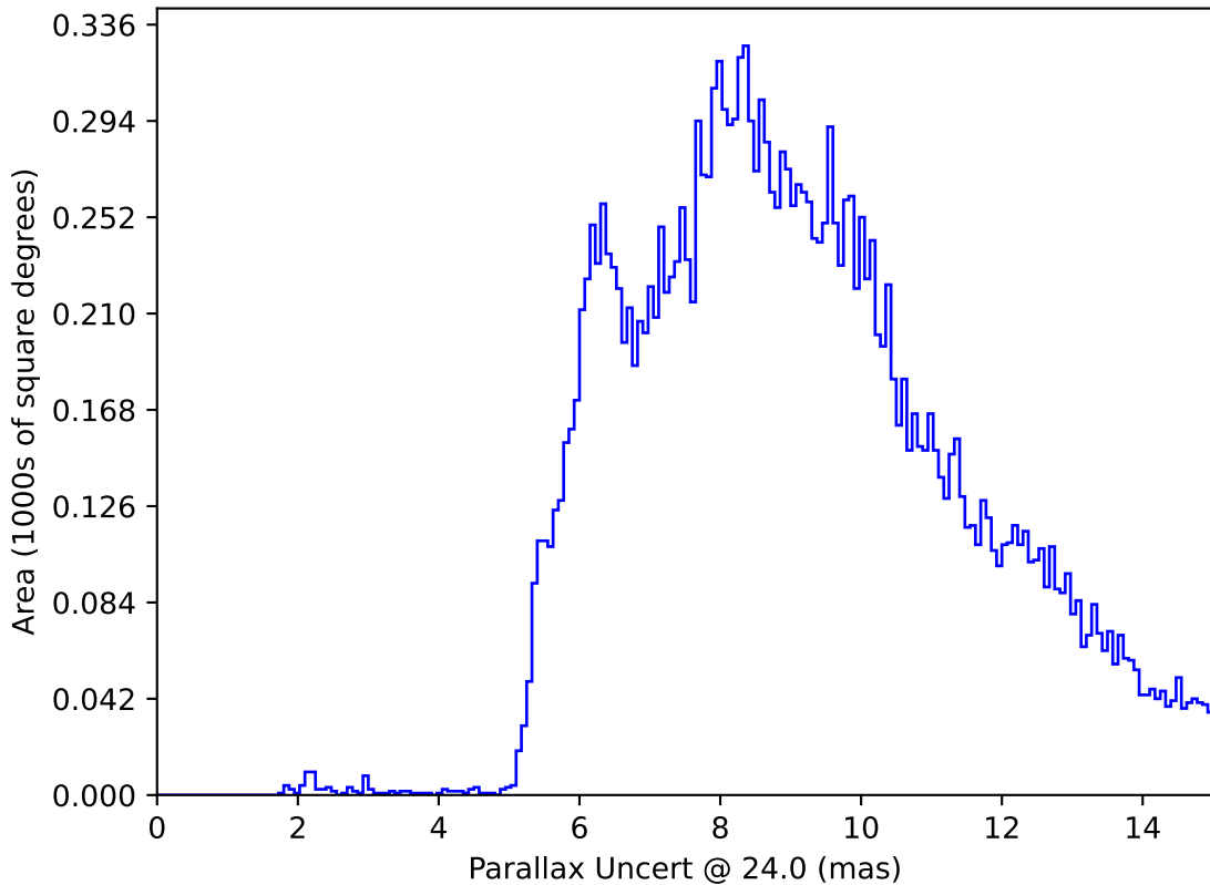
ddf_loaded_fl1_v3.3_10yrs : Parallax Uncert @ 24.0
