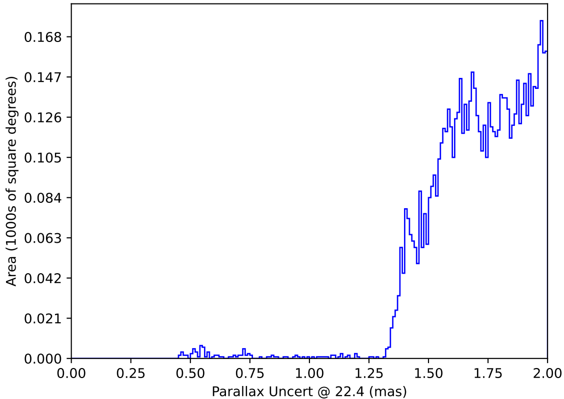
ddf_loaded_fl1_v3.3_10yrs : Parallax Uncert @ 22.4
